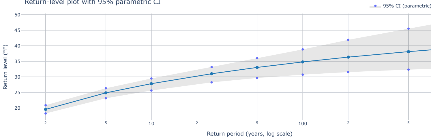
Return-level plot with 95% parametric CI
