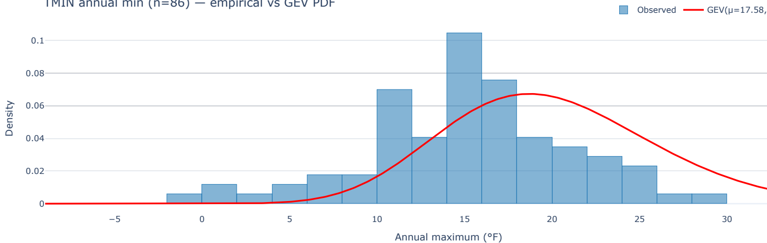
TMIN annual min (n=86) — empirical vs GEV PDF
