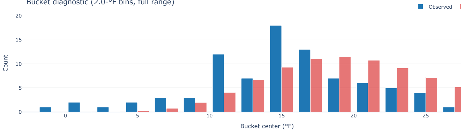
Bucket diagnostic (2.0-°F bins, full range)
